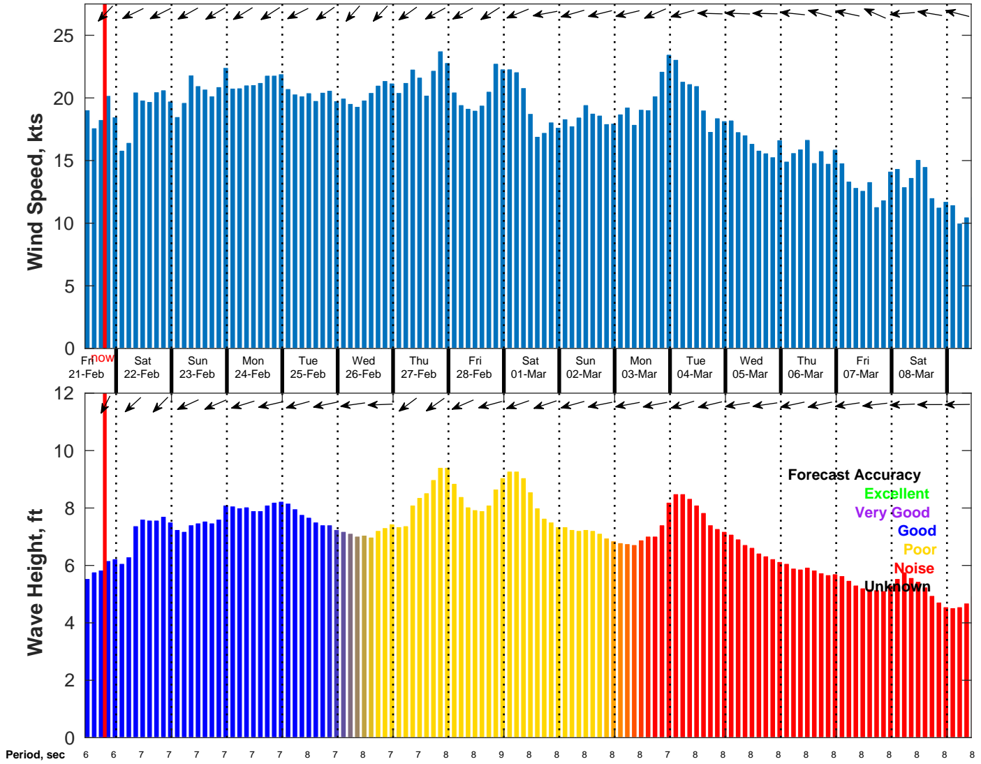
Wind & Wave Forecast for NDBC 52211 from 20-Feb-2025 10:00:00 to 08-Mar-2025 10:00:00
