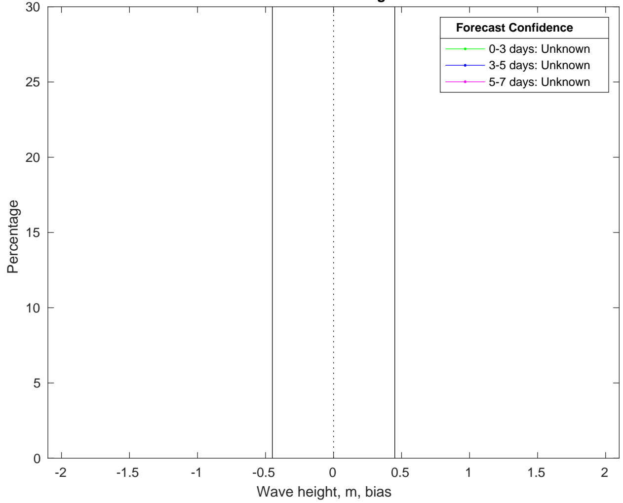
NDBC 52212 vs CMEMS Waves Bias Histogram: 20-Feb-2025
