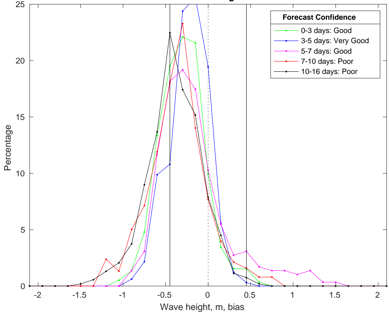
NDBC 52212 vs GFS Waves Bias Histogram: 20-Feb-2025
