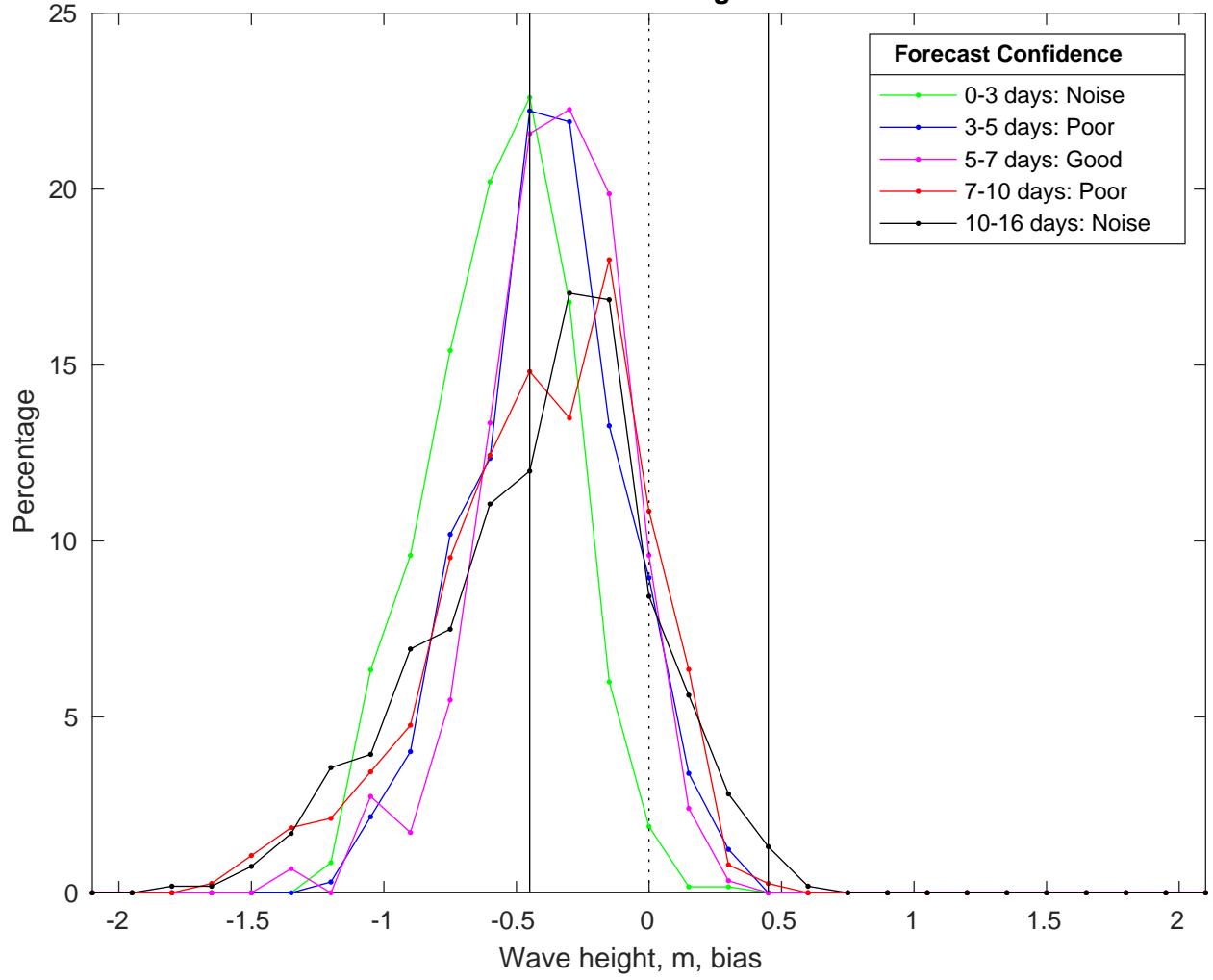
NDBC 52213 vs GFS Waves Bias Histogram: 20-Feb-2025
