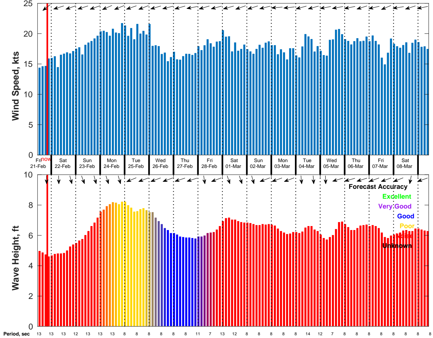
Wind & Wave Forecast for NDBC 52213 from 20-Feb-2025 11:00:00 to 08-Mar-2025 11:00:00
