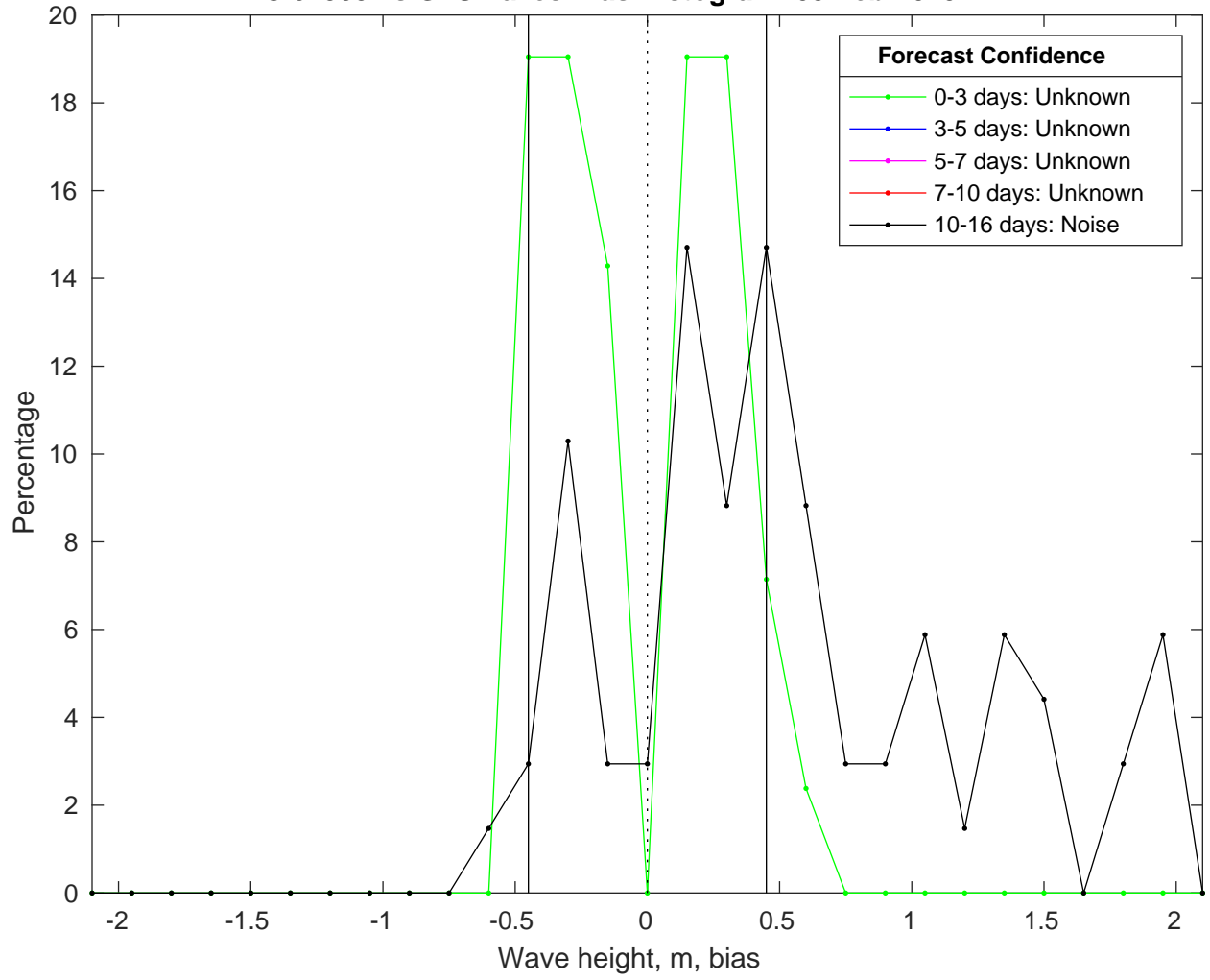
NDBC 62305 vs GFSWaves Bias Histogram: 03-Feb-2025
