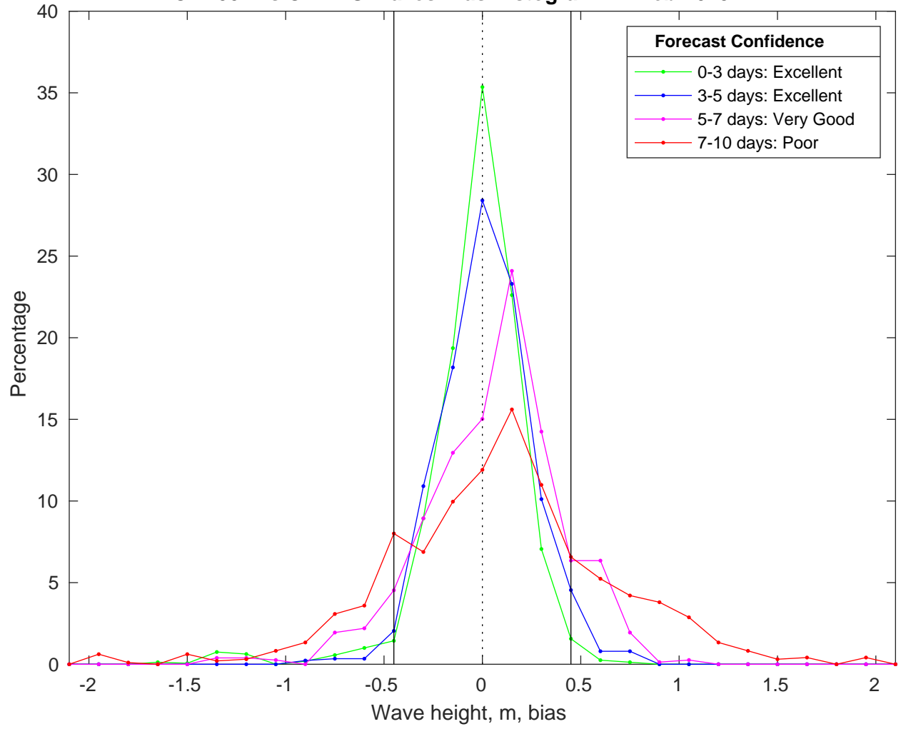
NDBC 41004 vs CMEMS Waves Bias Histogram: 21-Feb-2025
