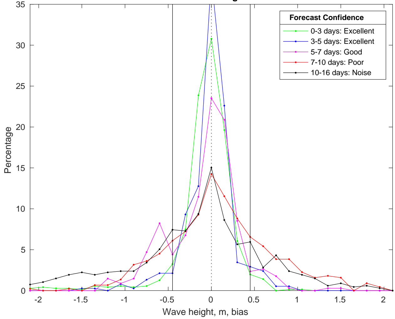
NDBC 41004 vs GFS Waves Bias Histogram: 21-Feb-2025
