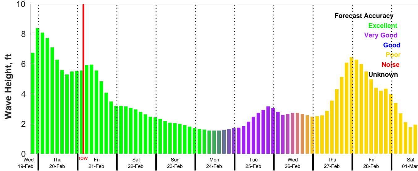
CMEMS Wave Forecast for NDBC 41004 from 19-Feb-2025 19:00:00 to 01-Mar-2025 19:00:00
