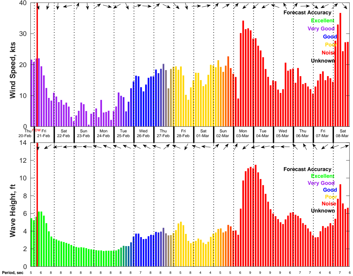
Wind & Wave Forecast for NDBC 41004 from 20-Feb-2025 19:00:00 to 08-Mar-2025 19:00:00
