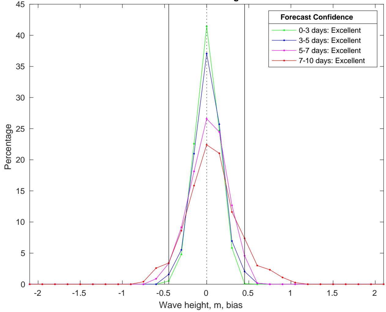
NDBC 41040 vs CMEMS Waves Bias Histogram: 21-Feb-2025
