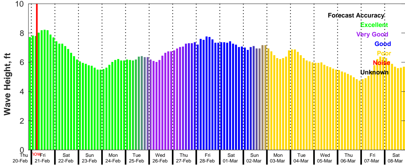
GFS Wave Forecast for NDBC 41040 from 20-Feb-2025 21:00:00 to 08-Mar-2025 21:00:00
