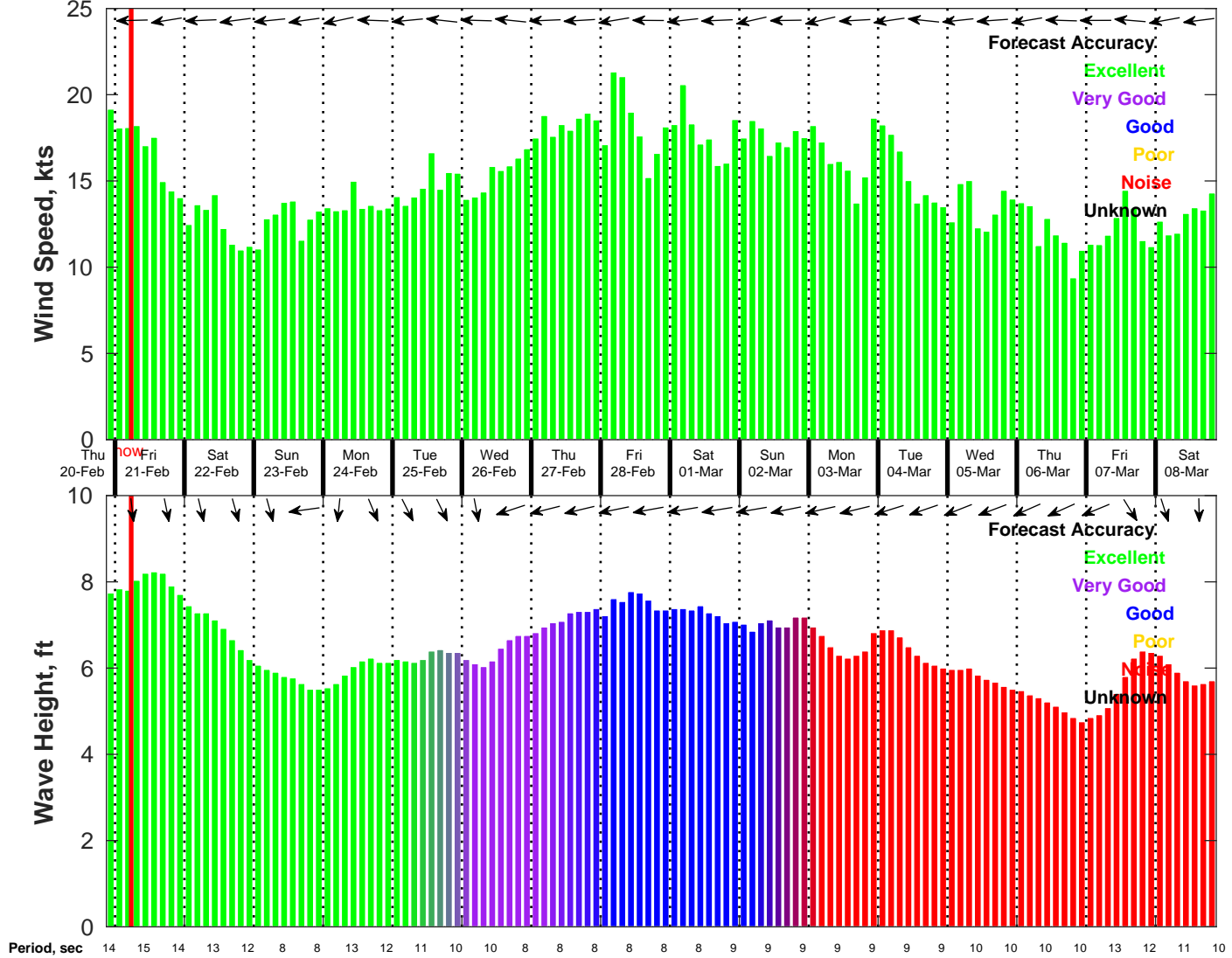
Wind & Wave Forecast for NDBC 41040 from 20-Feb-2025 21:00:00 to 08-Mar-2025 21:00:00
