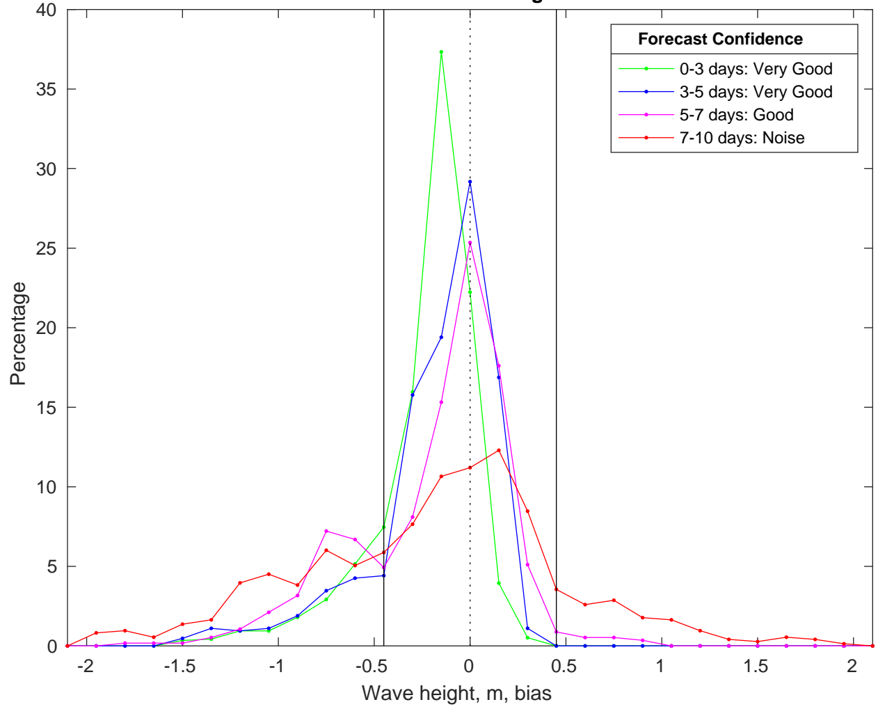
NDBC 42019 vs CMEMS Waves Bias Histogram: 21-Feb-2025
