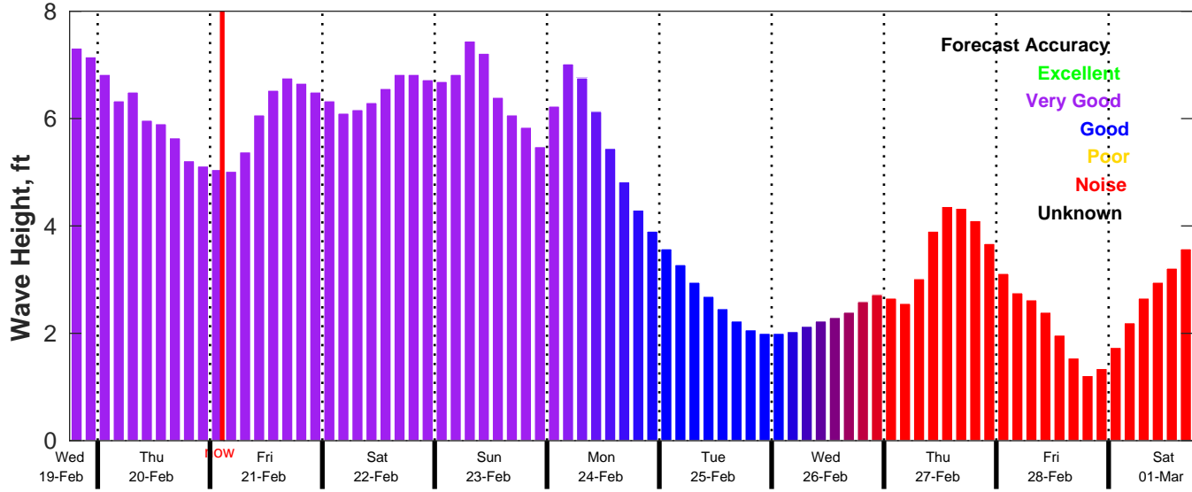
CMEMS Wave Forecast for NDBC 42019 from 19-Feb-2025 18:00:00 to 01-Mar-2025 18:00:00
