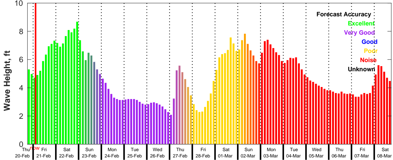
GFS Wave Forecast for NDBC 42019 from 20-Feb-2025 18:00:00 to 08-Mar-2025 18:00:00
