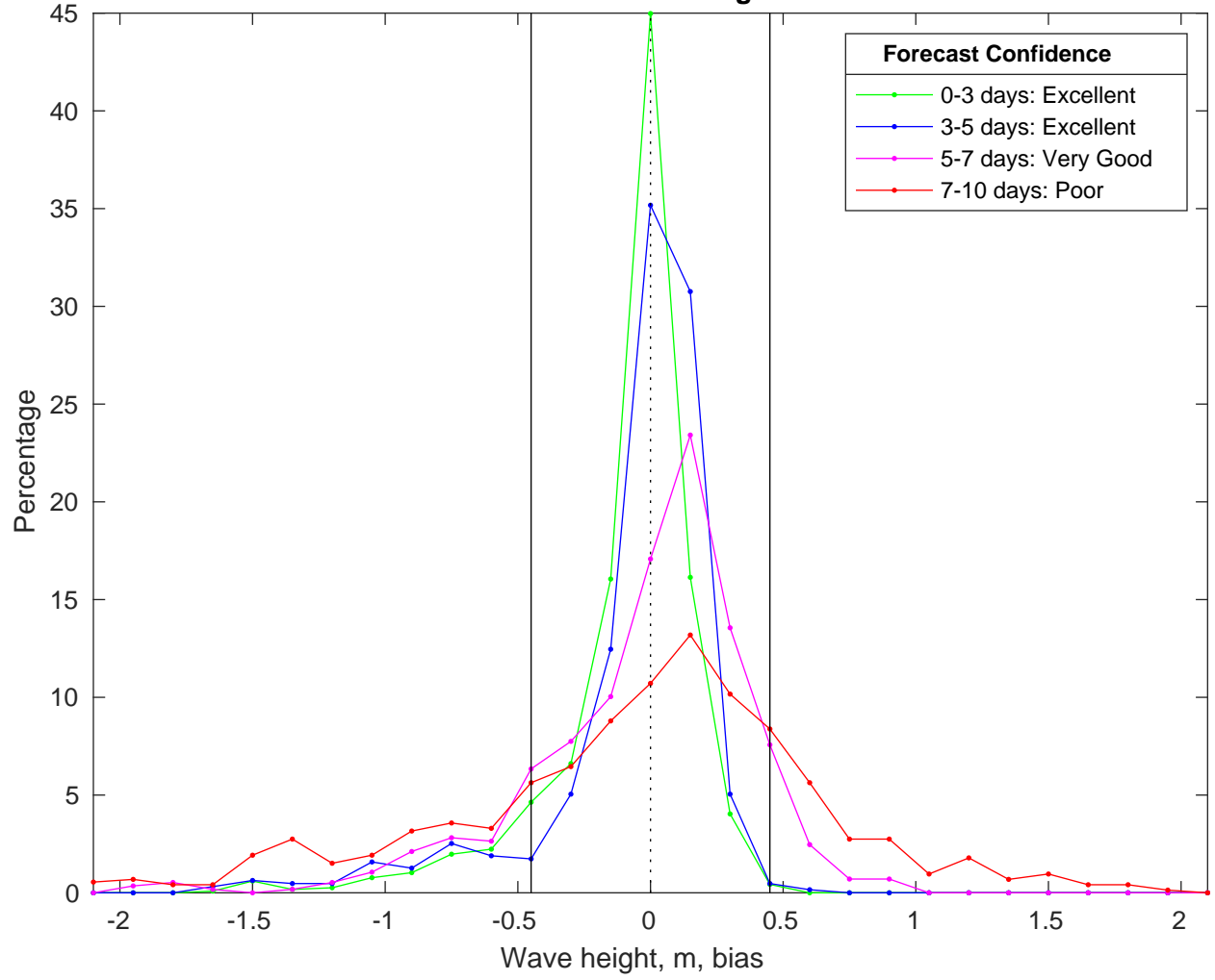
NDBC 42020 vs CMEMS Waves Bias Histogram: 21-Feb-2025
