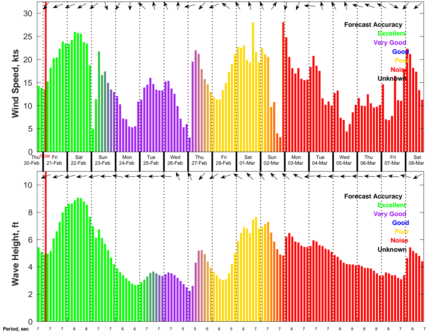
Wind & Wave Forecast for NDBC 42020 from 20-Feb-2025 18:00:00 to 08-Mar-2025 18:00:00
