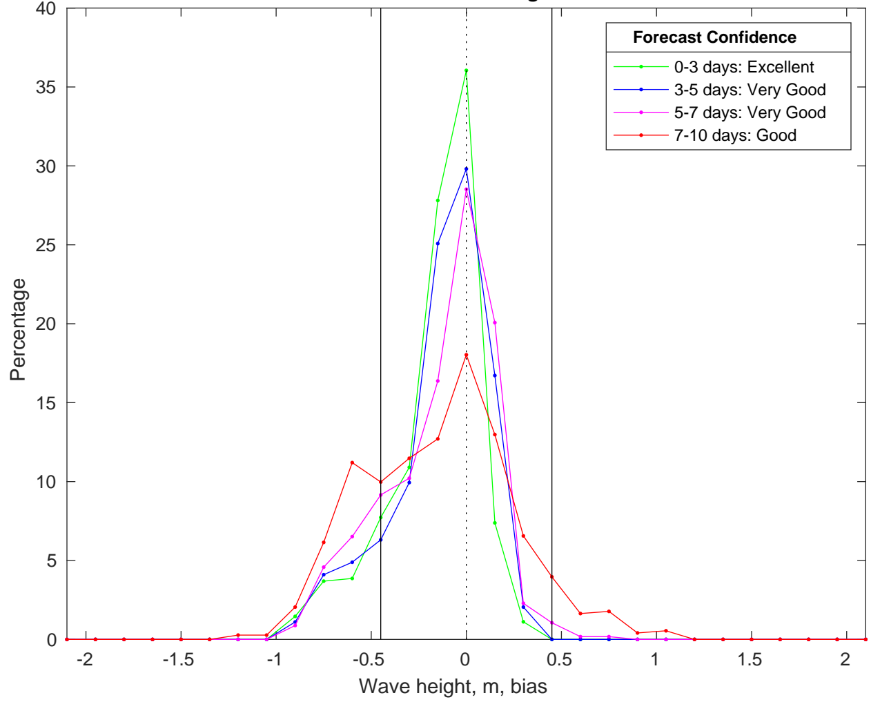
NDBC 42035 vs CMEMS Waves Bias Histogram: 21-Feb-2025
