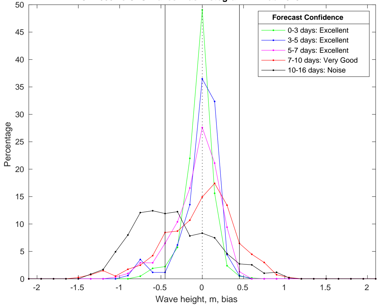
NDBC 42035 vs GFS Waves Bias Histogram: 21-Feb-2025
