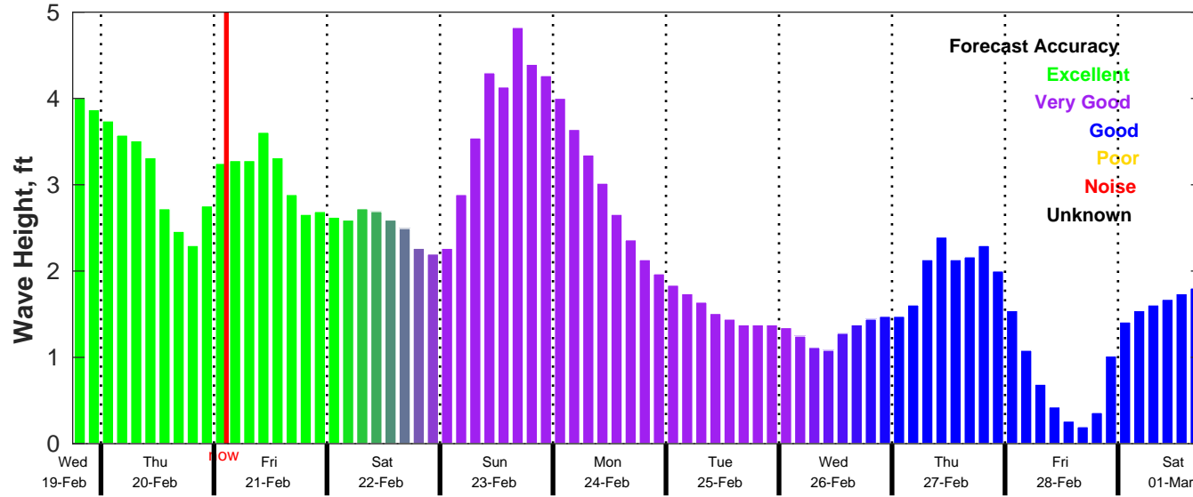
CMEMS Wave Forecast for NDBC 42035 from 19-Feb-2025 18:00:00 to 01-Mar-2025 18:00:00
