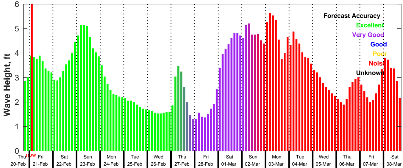
GFS Wave Forecast for NDBC 42035 from 20-Feb-2025 18:00:00 to 08-Mar-2025 18:00:00
