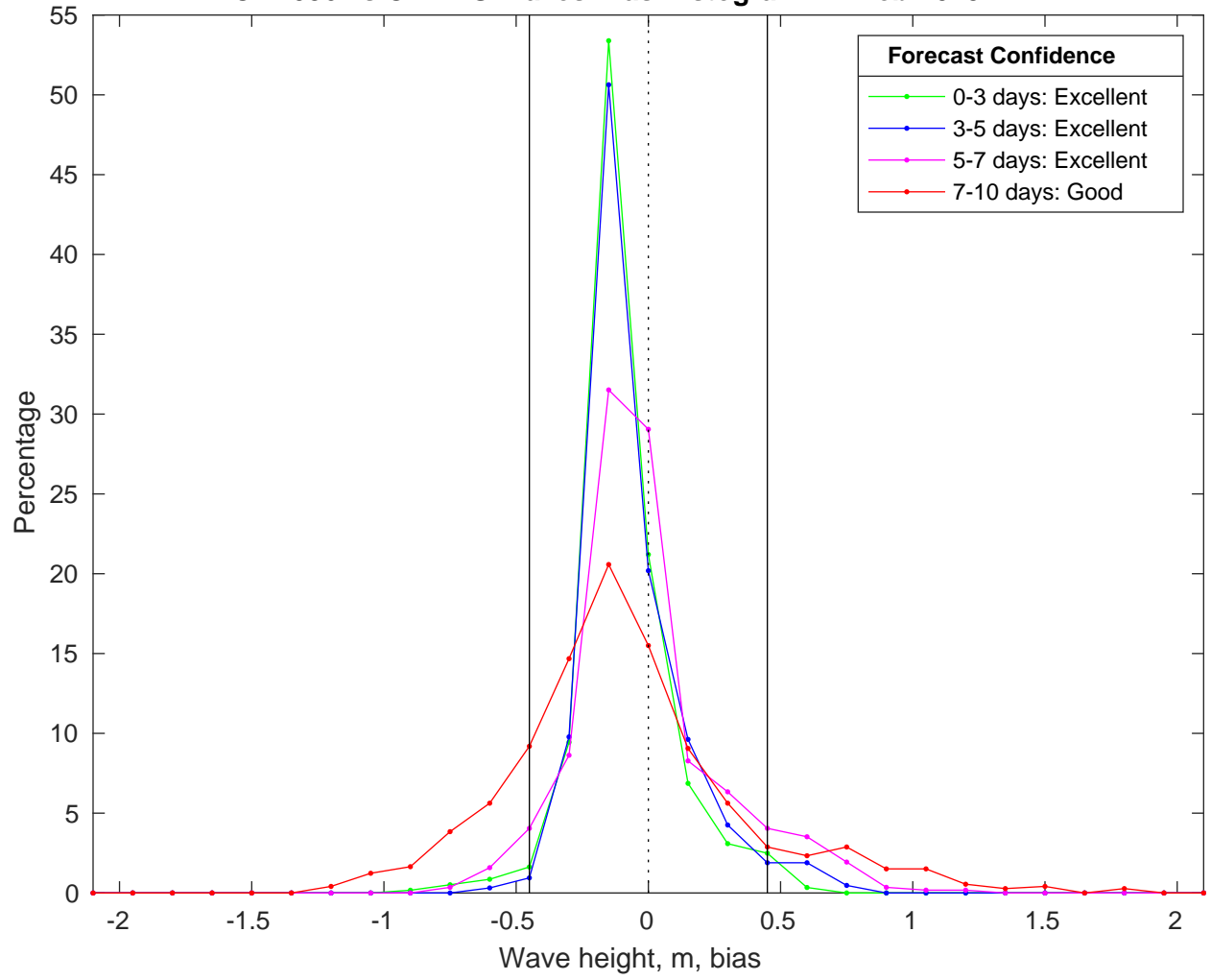
NDBC 42036 vs CMEMS Waves Bias Histogram: 21-Feb-2025
