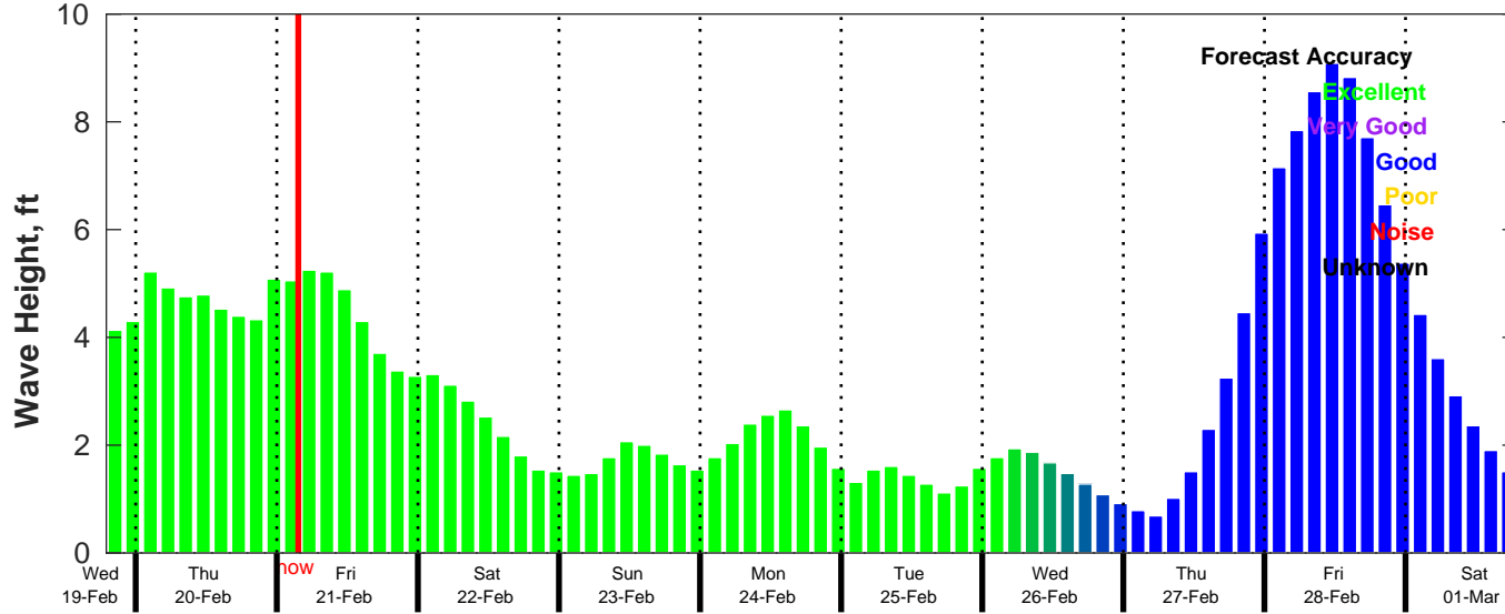
CMEMS Wave Forecast for NDBC 42036 from 19-Feb-2025 19:00:00 to 01-Mar-2025 19:00:00
