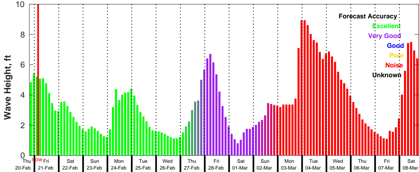
GFS Wave Forecast for NDBC 42036 from 20-Feb-2025 19:00:00 to 08-Mar-2025 19:00:00
