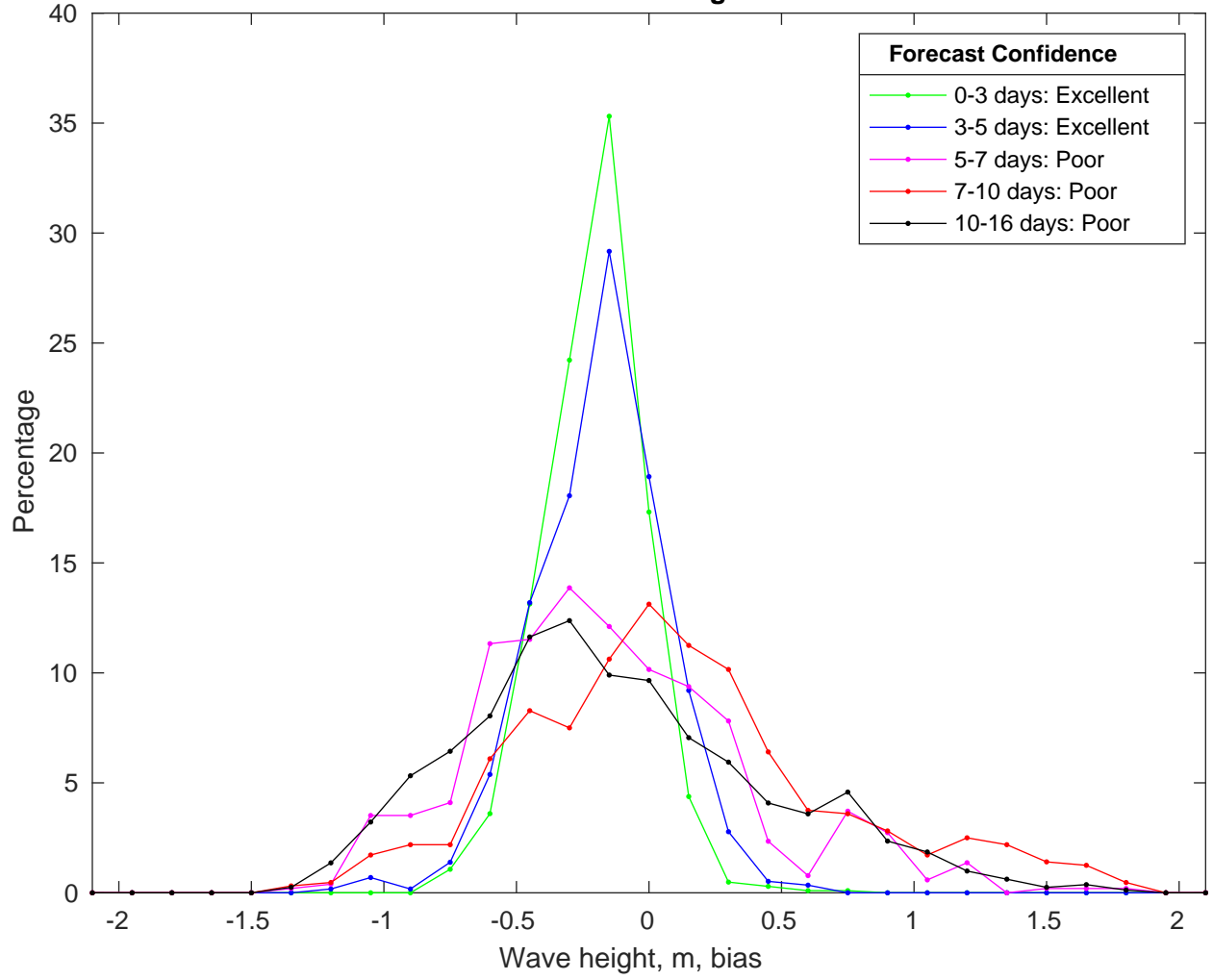
NDBC 42036 vs GFSWaves Bias Histogram: 26-Dec-2024
