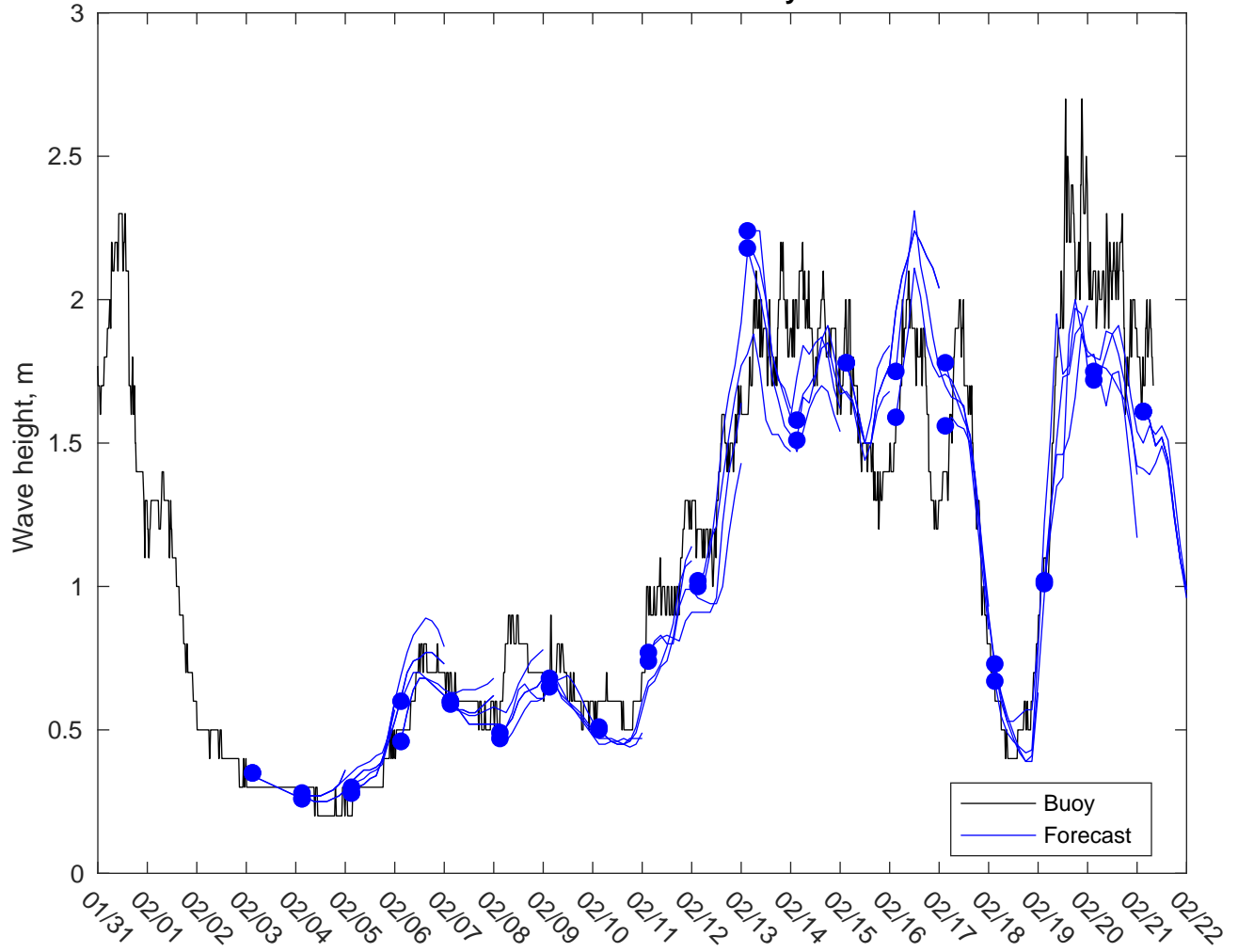
NDBC 42040 vs CMEMS Waves: 3 to 5 day forecast
