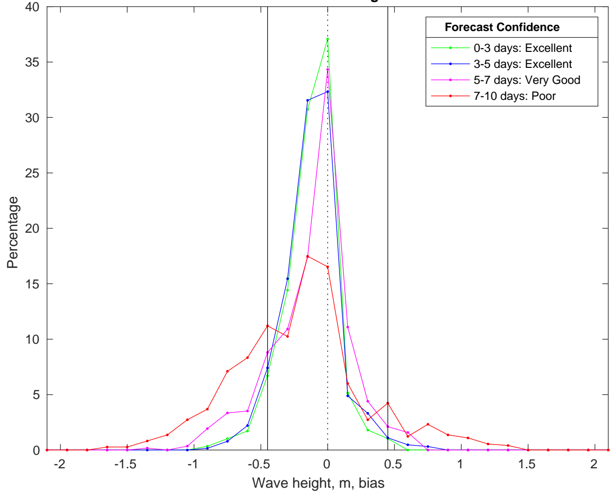
NDBC 42040 vs CMEMS Waves Bias Histogram: 21-Feb-2025
