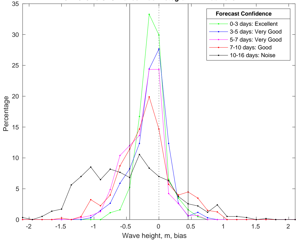
NDBC 42040 vs GFS Waves Bias Histogram: 21-Feb-2025
