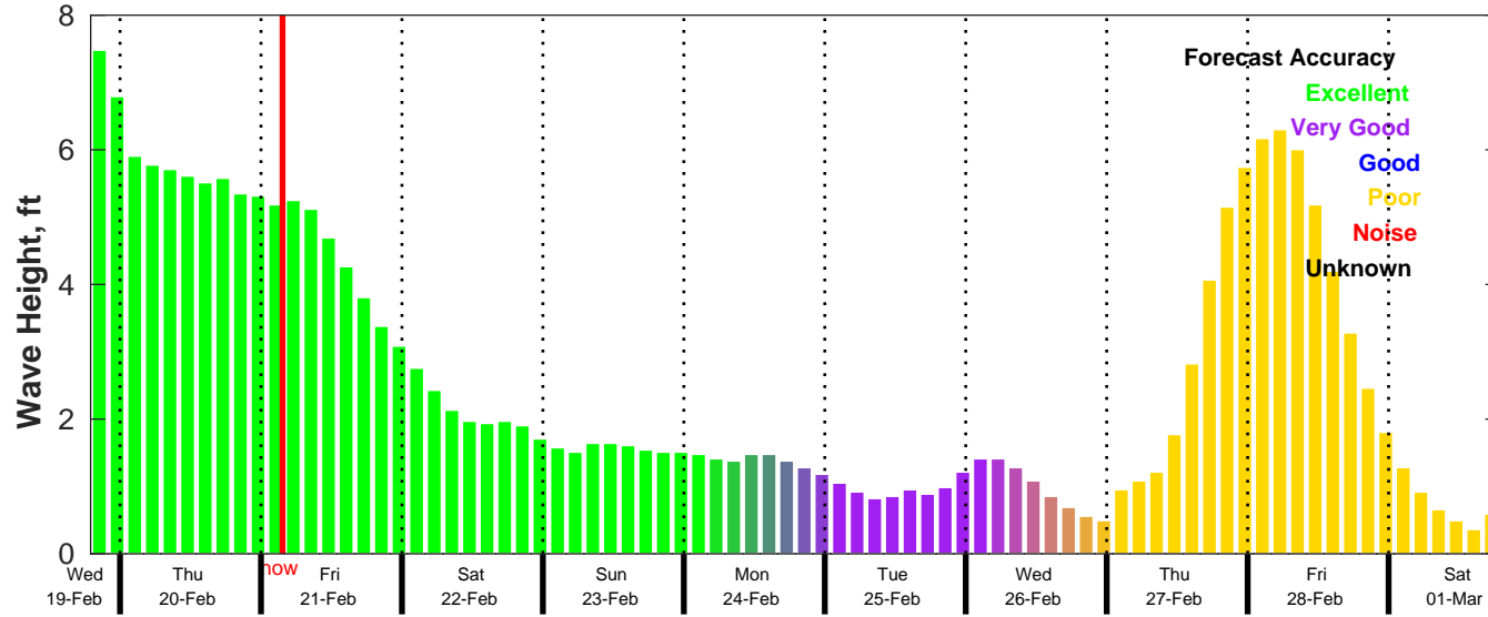
CMEMS Wave Forecast for NDBC 42040 from 19-Feb-2025 19:00:00 to 01-Mar-2025 19:00:00
