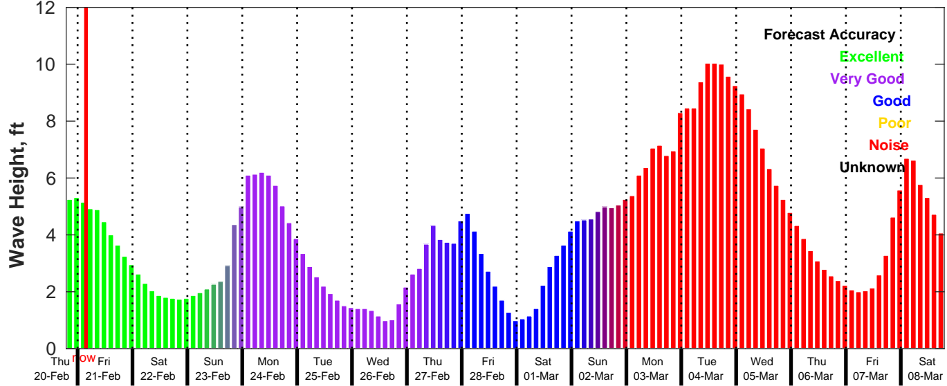
GFS Wave Forecast for NDBC 42040 from 20-Feb-2025 19:00:00 to 08-Mar-2025 19:00:00
