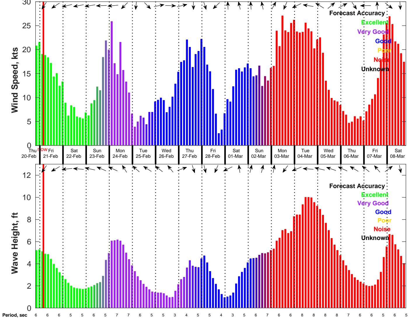
Wind & Wave Forecast for NDBC 42040 from 20-Feb-2025 19:00:00 to 08-Mar-2025 19:00:00
