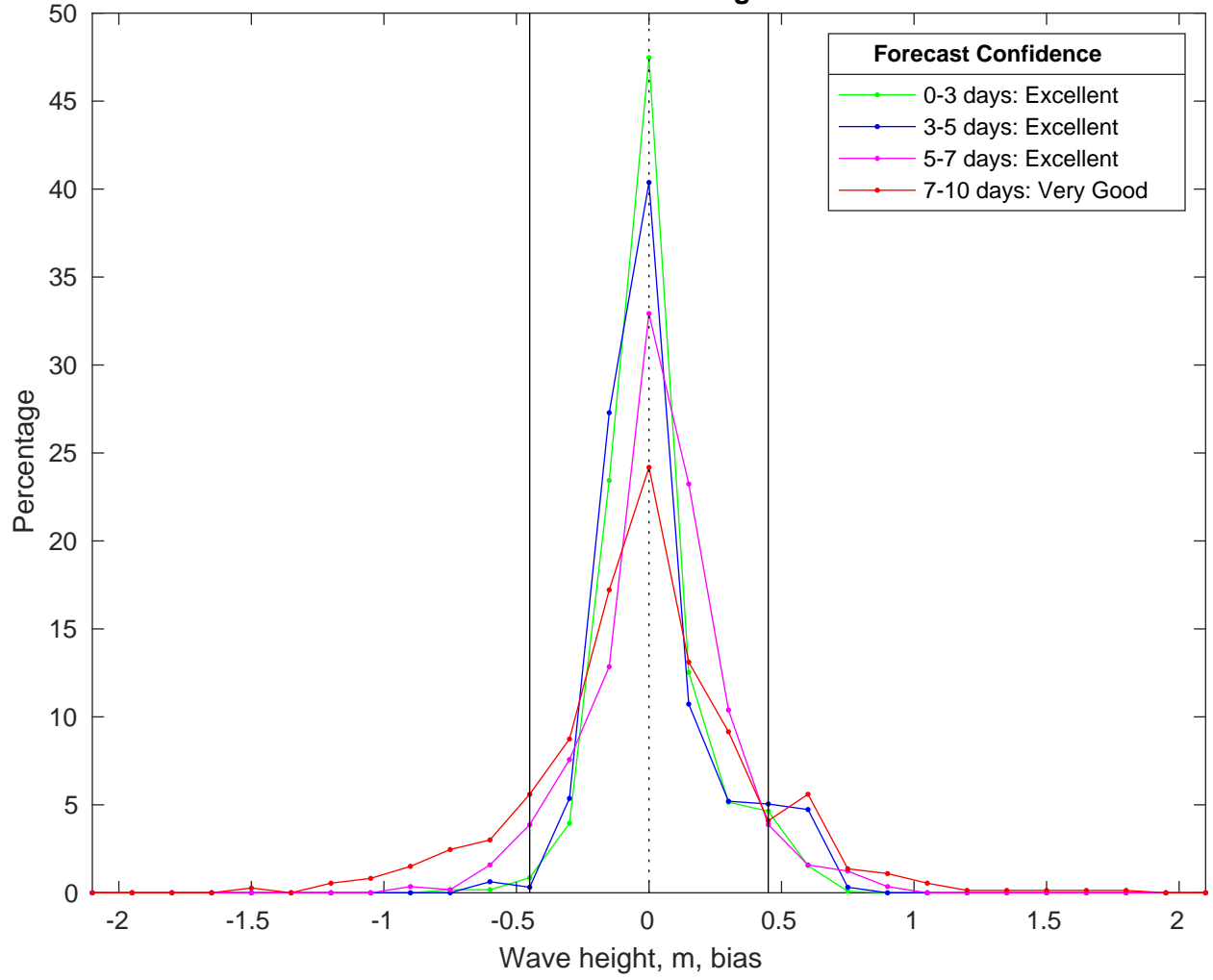
NDBC 42084 vs CMEMS Waves Bias Histogram: 21-Feb-2025
