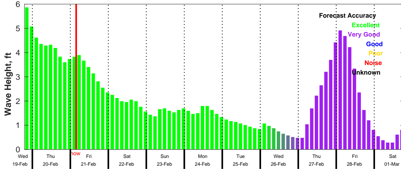
CMEMS Wave Forecast for NDBC 42084 from 19-Feb-2025 19:00:00 to 01-Mar-2025 19:00:00
