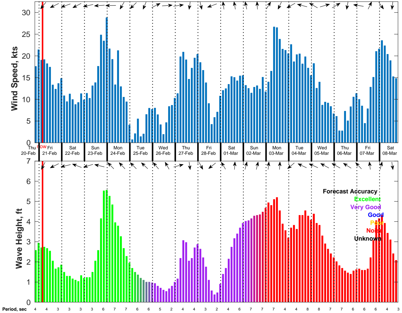
Wind & Wave Forecast for NDBC 42084 from 20-Feb-2025 19:00:00 to 08-Mar-2025 19:00:00
