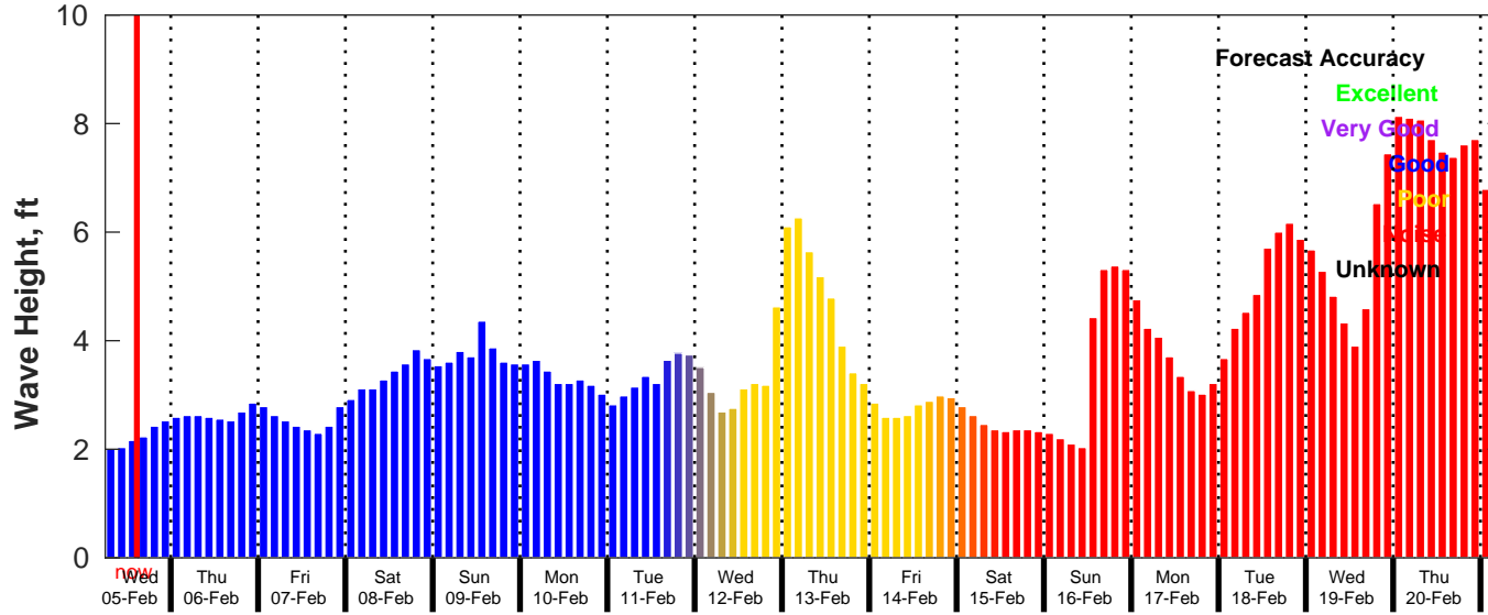
GFS Wave Forecast for NDBC 42092 from 05-Feb-2025 06:00:00 to 21-Feb-2025 06:00:00
