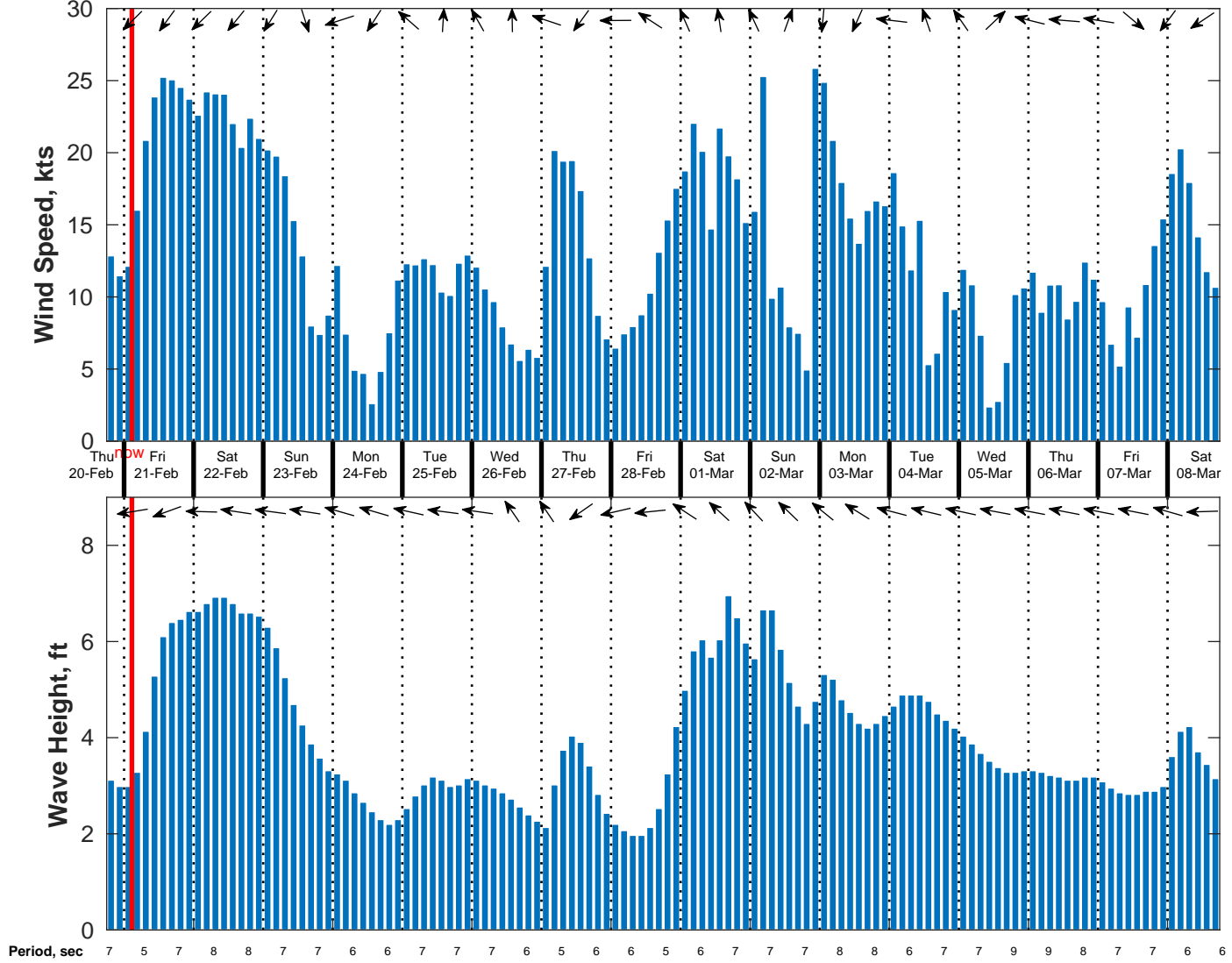
Wind & Wave Forecast for NDBC 42092 from 20-Feb-2025 18:00:00 to 08-Mar-2025 18:00:00
