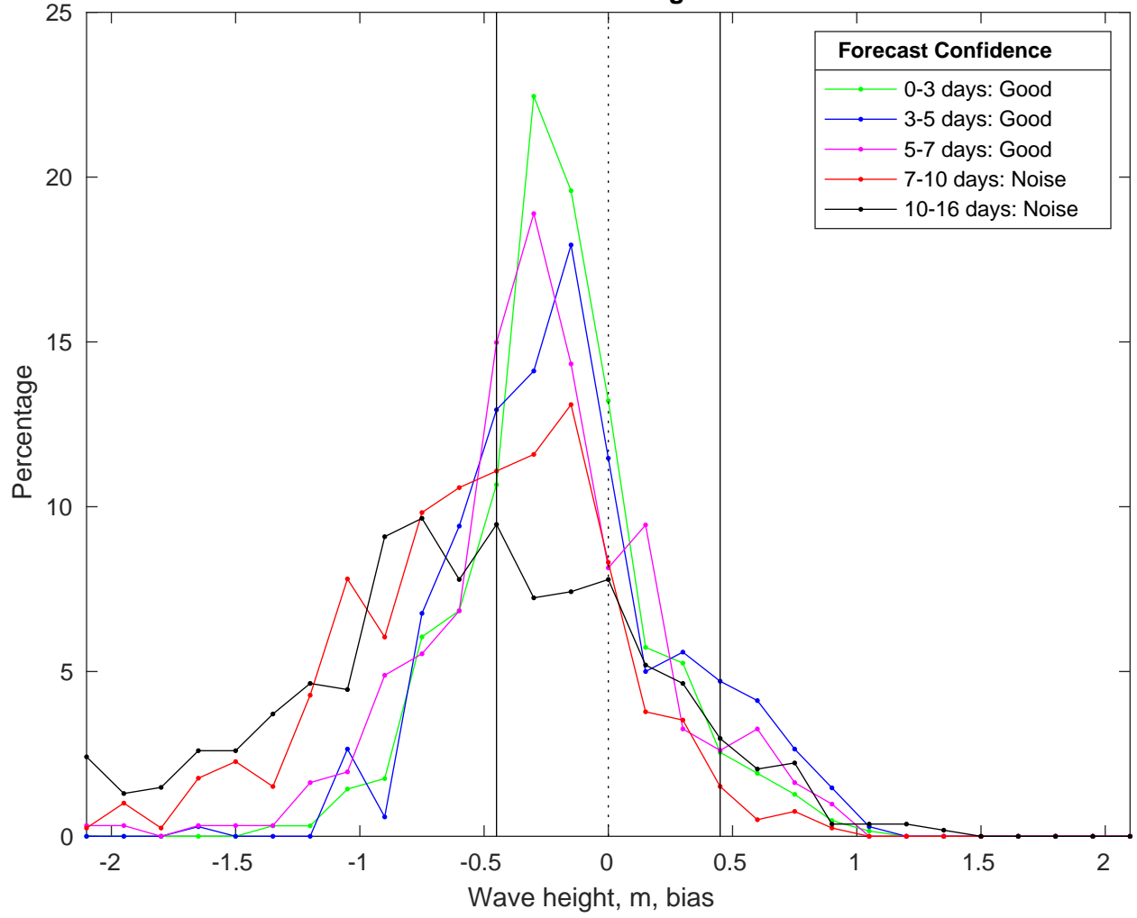
NDBC 46011 vs GFS Waves Bias Histogram: 21-Feb-2025
