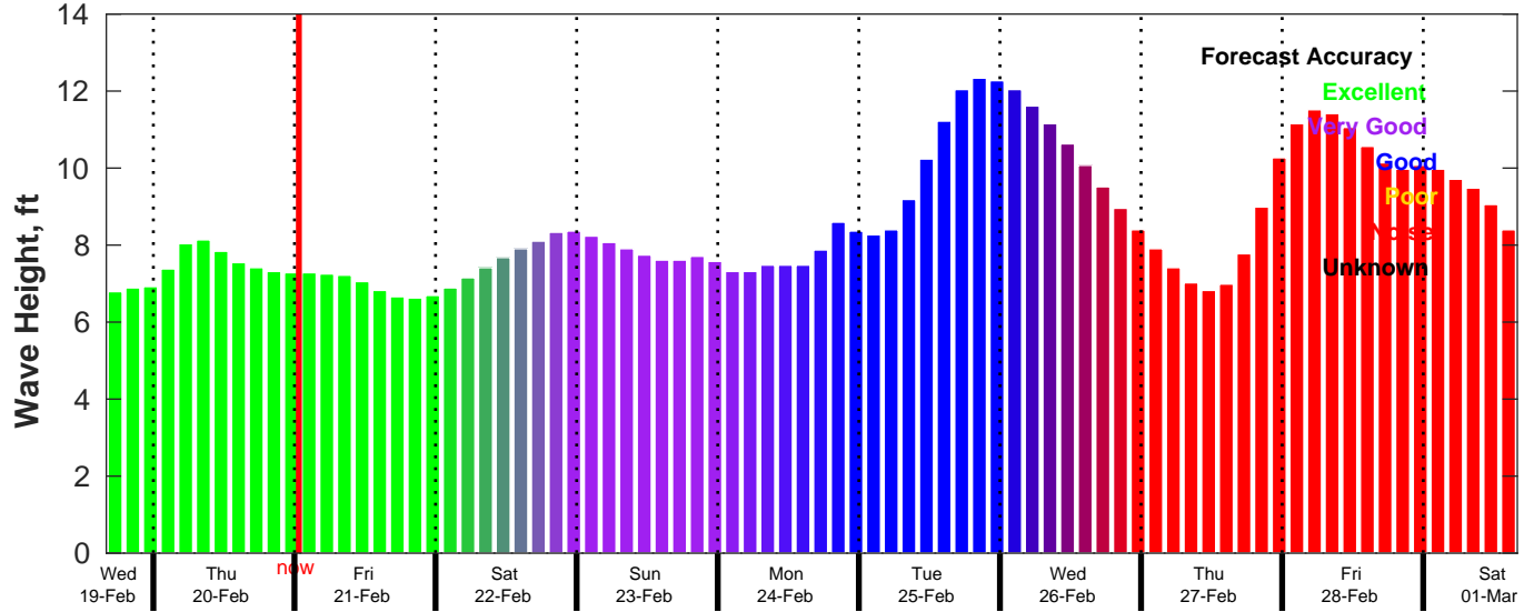
CMEMS Wave Forecast for NDBC 46011 from 19-Feb-2025 16:00:00 to 01-Mar-2025 16:00:00
