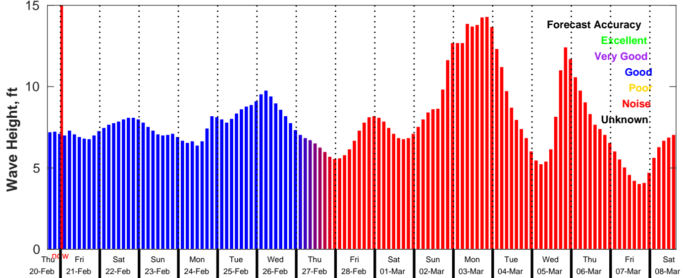
GFS Wave Forecast for NDBC 46011 from 20-Feb-2025 16:00:00 to 08-Mar-2025 16:00:00
