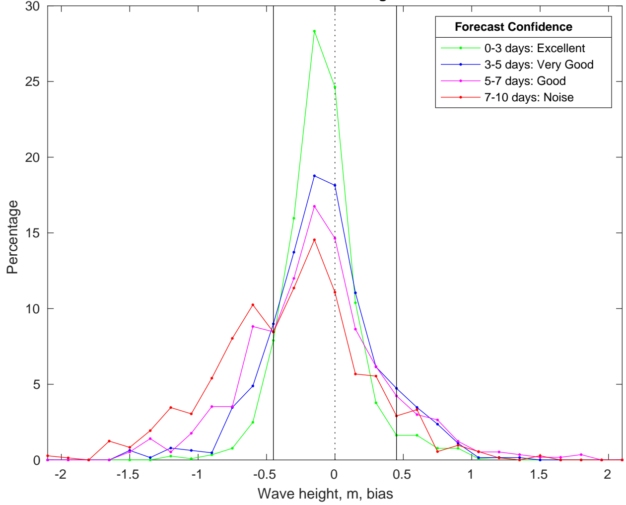
NDBC 46028 vs CMEMS Waves Bias Histogram: 21-Feb-2025
