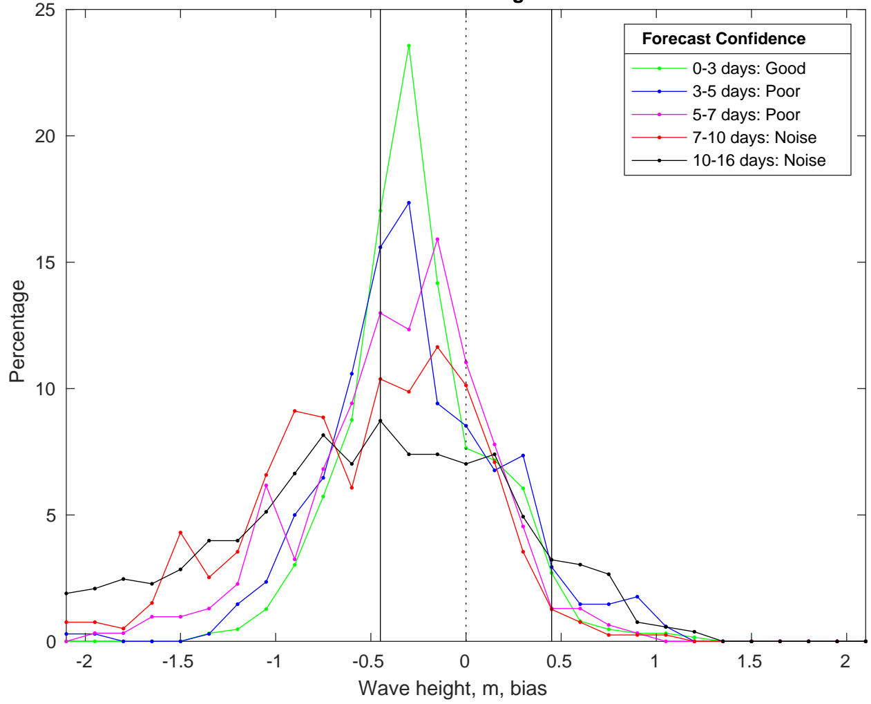
NDBC 46028 vs GFS Waves Bias Histogram: 21-Feb-2025
