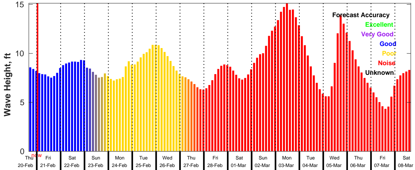
GFS Wave Forecast for NDBC 46028 from 20-Feb-2025 16:00:00 to 08-Mar-2025 16:00:00
