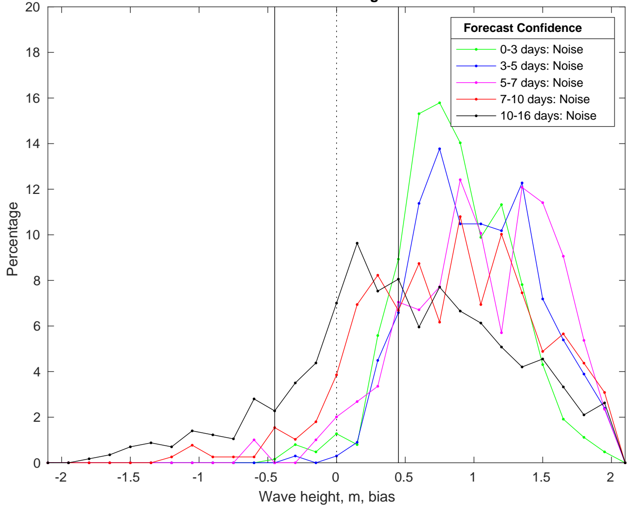
NDBC 46053 vs GFS Waves Bias Histogram: 21-Feb-2025
