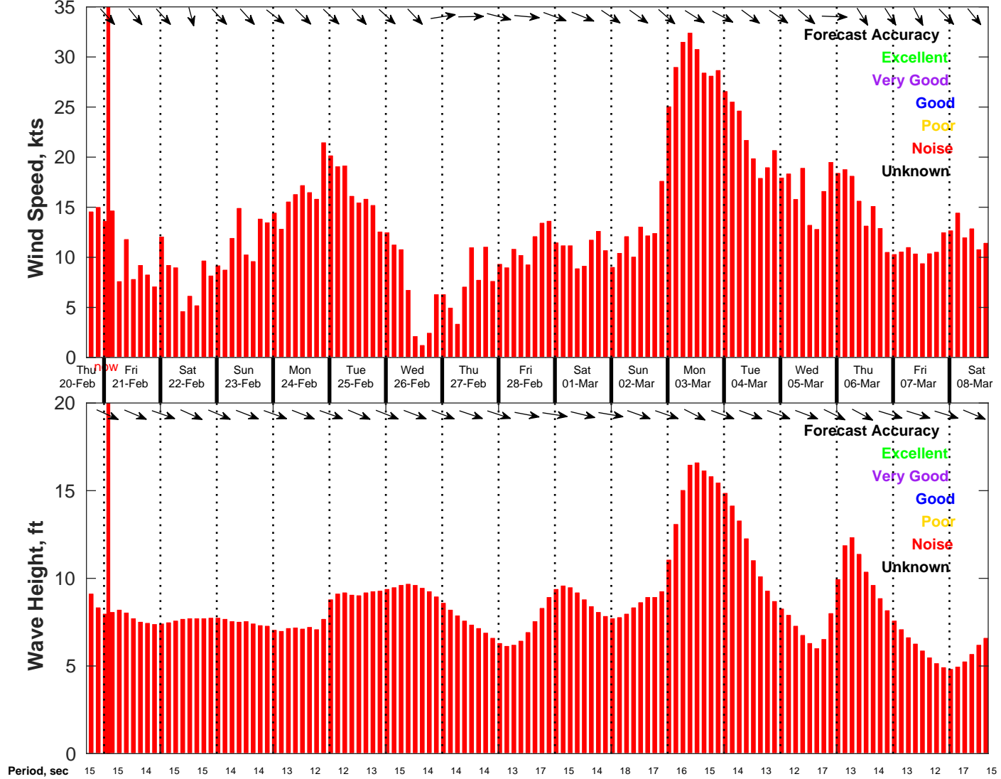
Wind & Wave Forecast for NDBC 46053 from 20-Feb-2025 17:00:00 to 08-Mar-2025 17:00:00
