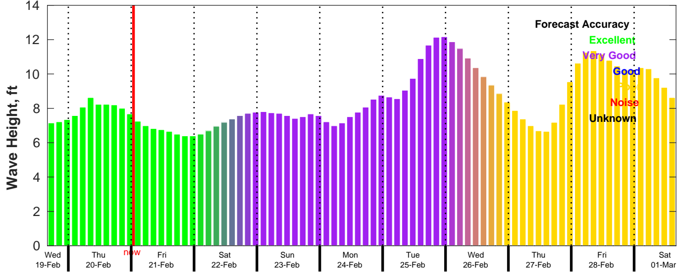
CMEMS Wave Forecast for NDBC 46054 from 19-Feb-2025 16:00:00 to 01-Mar-2025 16:00:00
