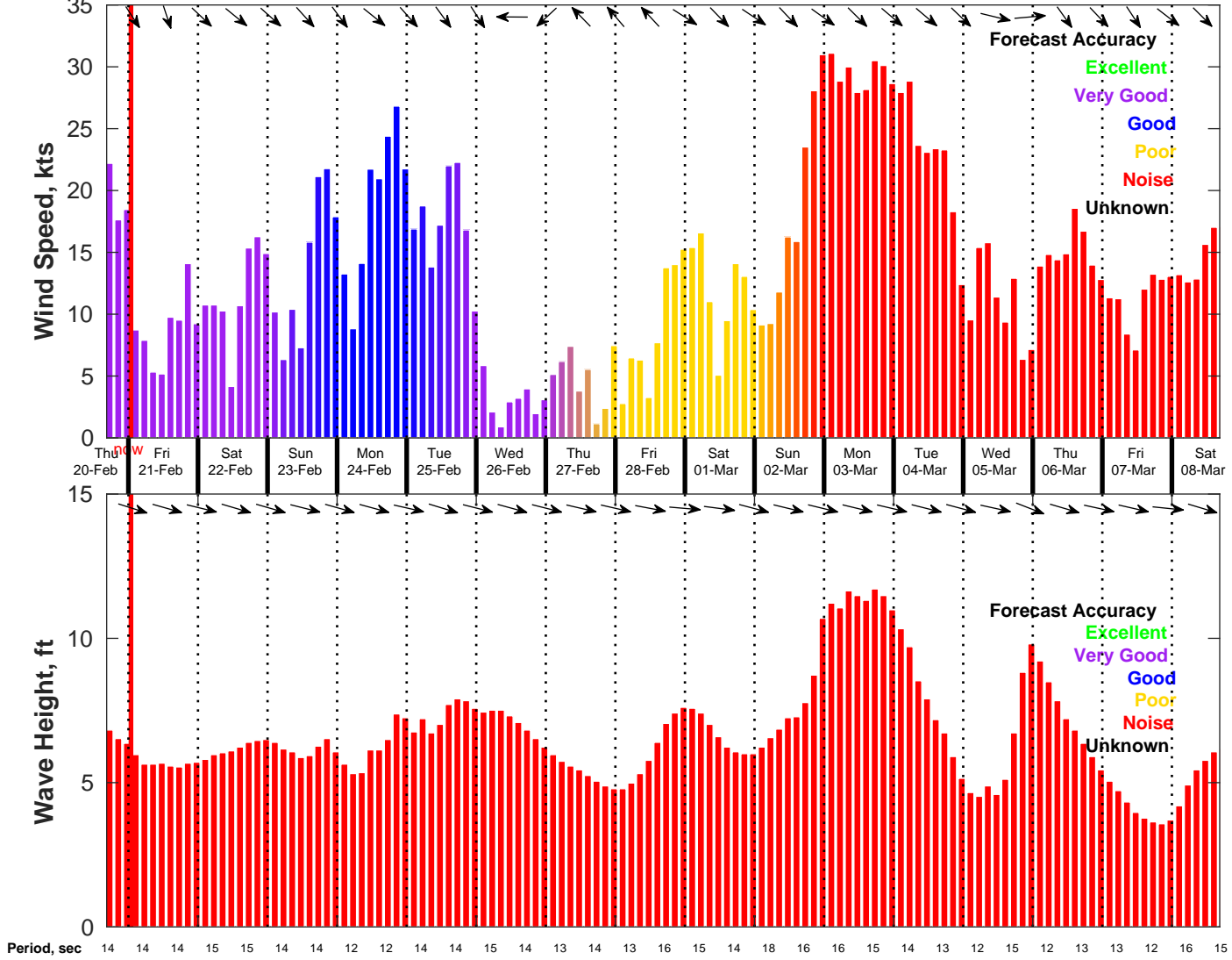
Wind & Wave Forecast for NDBC 46054 from 20-Feb-2025 16:00:00 to 08-Mar-2025 16:00:00
