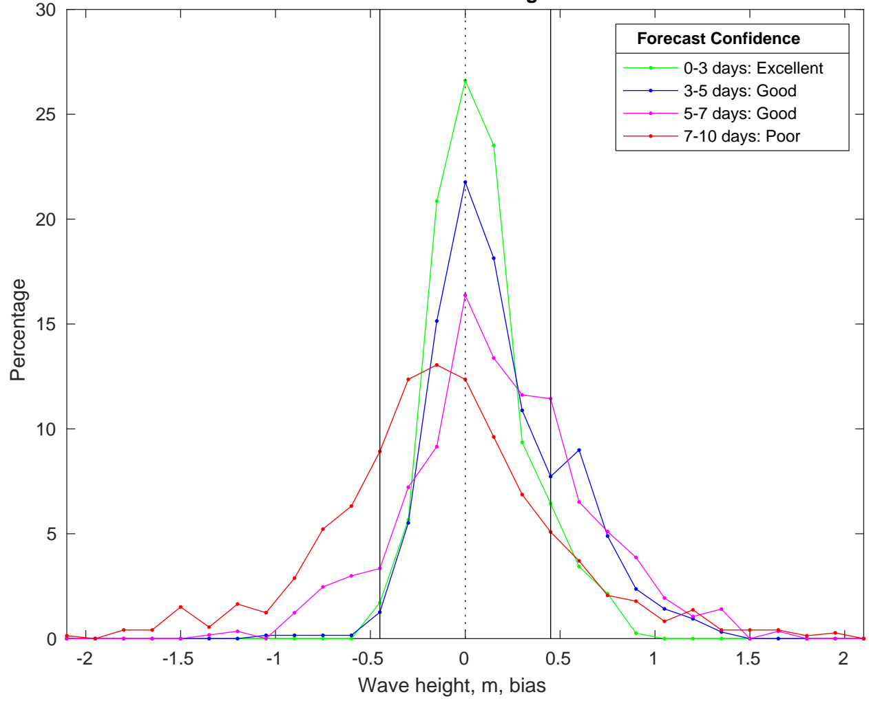
NDBC 46069 vs CMEMS Waves Bias Histogram: 21-Feb-2025
