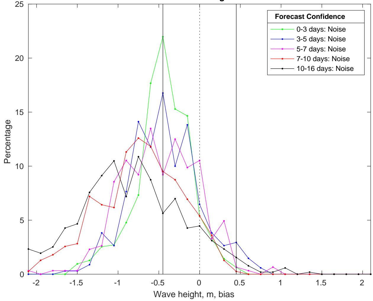
NDBC 46069 vs GFS Waves Bias Histogram: 21-Feb-2025
