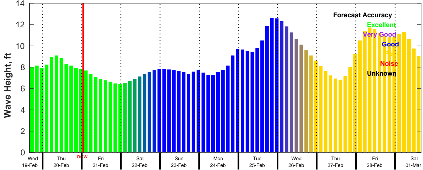
CMEMS Wave Forecast for NDBC 46069 from 19-Feb-2025 16:00:00 to 01-Mar-2025 16:00:00
